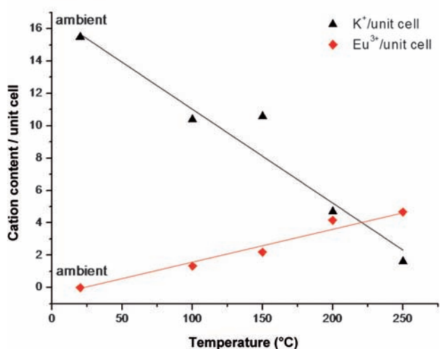
Figure 4. SEM/EDX elemental analysis data for quenched samples from a) isothermal high-pressure runs performed at 150^\circ\text{C} and b) isobaric high-pressure runs performed at 3.0 GPa. Solid lines are guides to the eyes. Estimated standard deviations are smaller than the symbols.
